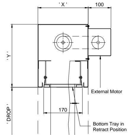
HEADBOX DETAIL
