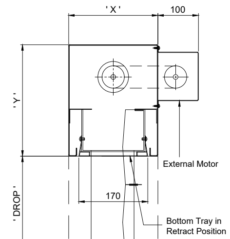
HEADBOX DETAIL
