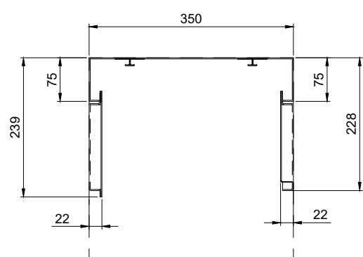
DOOR OPENED
