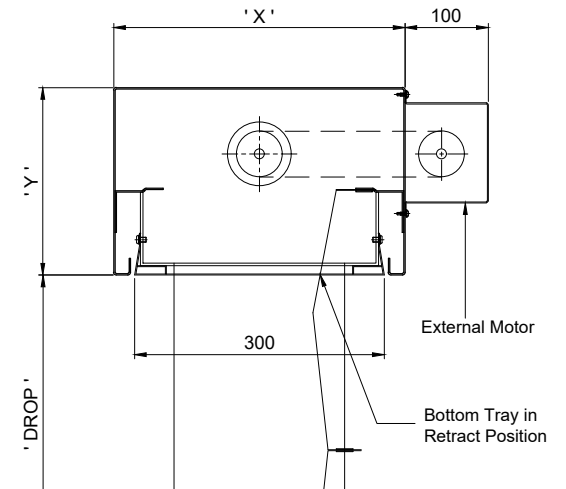
HEADBOX DETAIL
