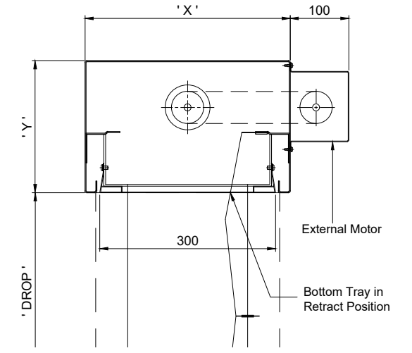
HEADBOX DETAIL
