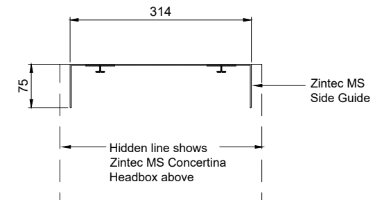
SIDE GUIDE DETAIL
