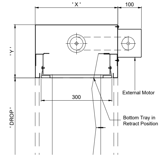
HEADBOX DETAIL
