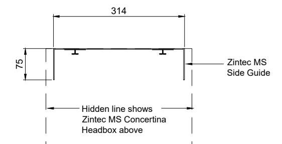
SIDE GUIDE DETAIL
