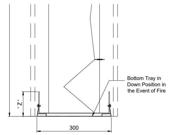
BOTTOM TRAY DETAIL SECTION A
