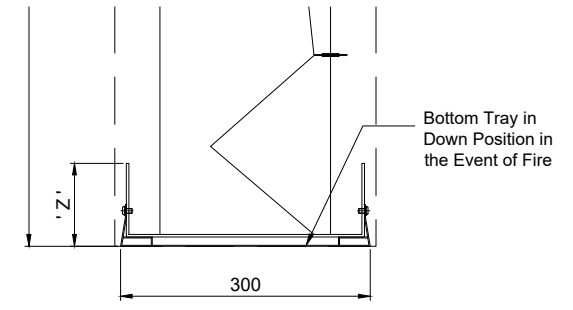
BOTTOM TRAY DETAIL SECTION A
