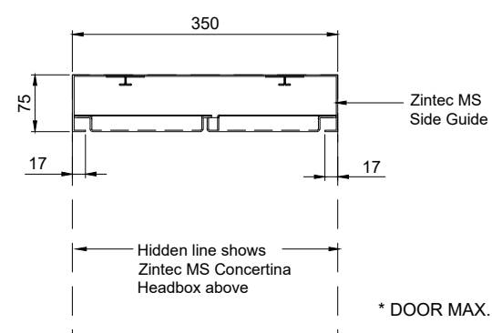
DOOR CLOSED
