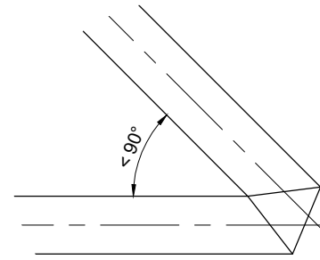
LESS THAN 90 DEG DETAIL
