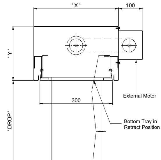
HEADBOX DETAIL
