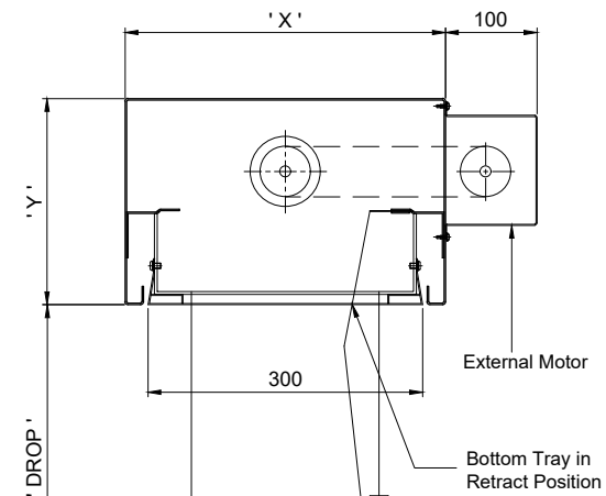
HEADBOX DETAIL
