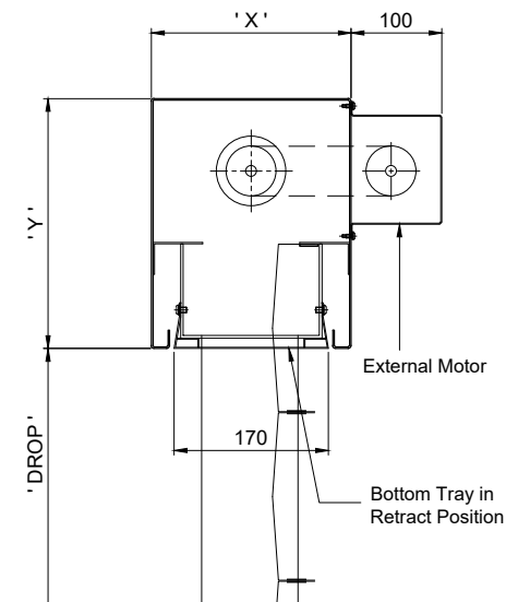
HEADBOX DETAIL
