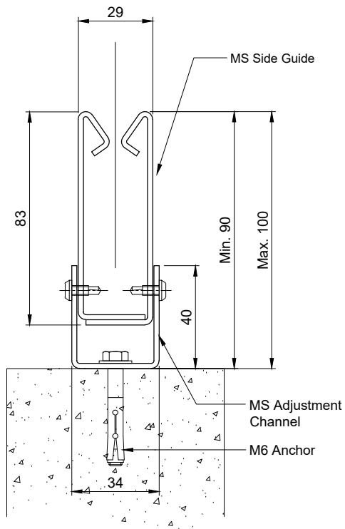
SIDE MOUNTED SIDE GUIDE DETAILS
