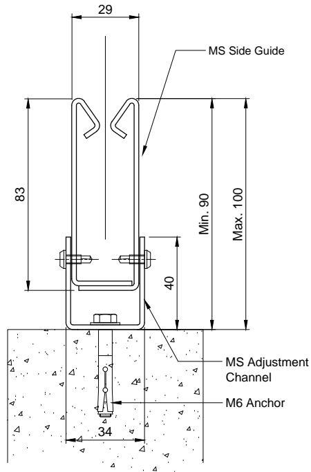
SIDE MOUNTED SIDE GUIDE DETAILS
