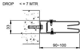
SIDE FIX
